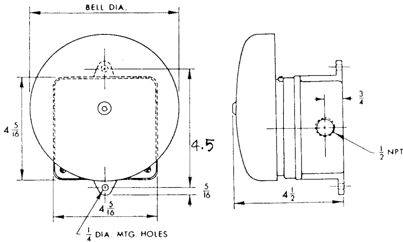
WEATHERPROOF BELL
