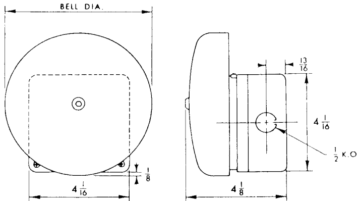
GENERAL PURPOSE BELL
