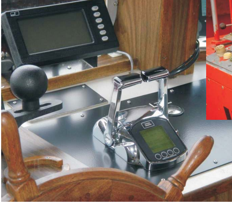
Seaspan Cates 6 Ship Assist Tug retrofitted with new MTU 8V4000 engines. The existing MG-540 gearboxes were modified for electric control
